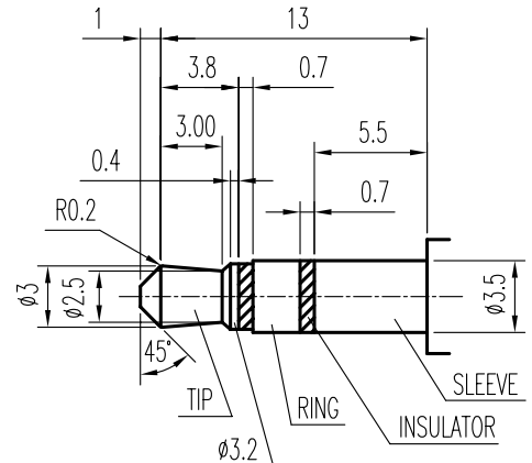
MATE PLUG
