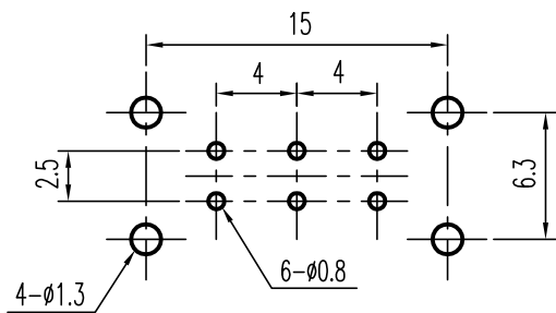
PIERCING PLAN
